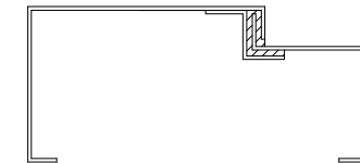
Single Rabbet Thermal Break (SRTB)
