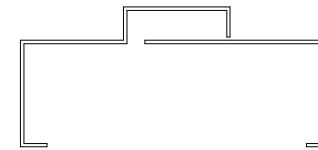
Double Rabbet Split (DRS)
