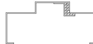
Double Rabbet Thermal Break (DRTB)
